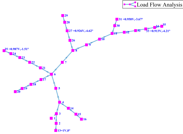
Fig. 19. System Topology.
